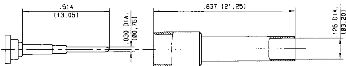
CENTER CONTACT SUB ASSEMBLY
